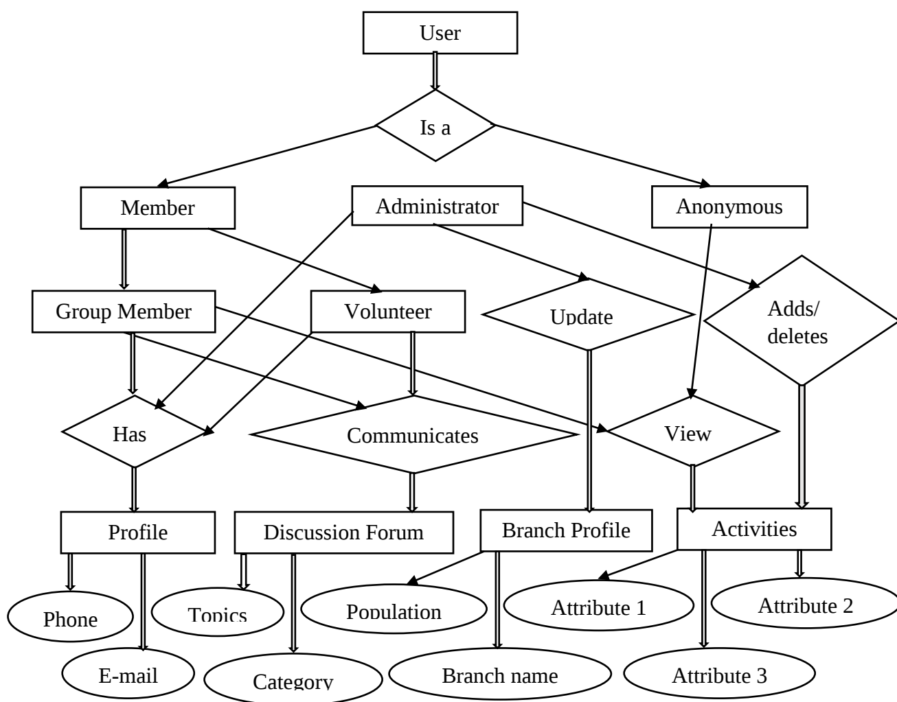
Figure 3.5: Entity Relationship Model Among All Perimeters
