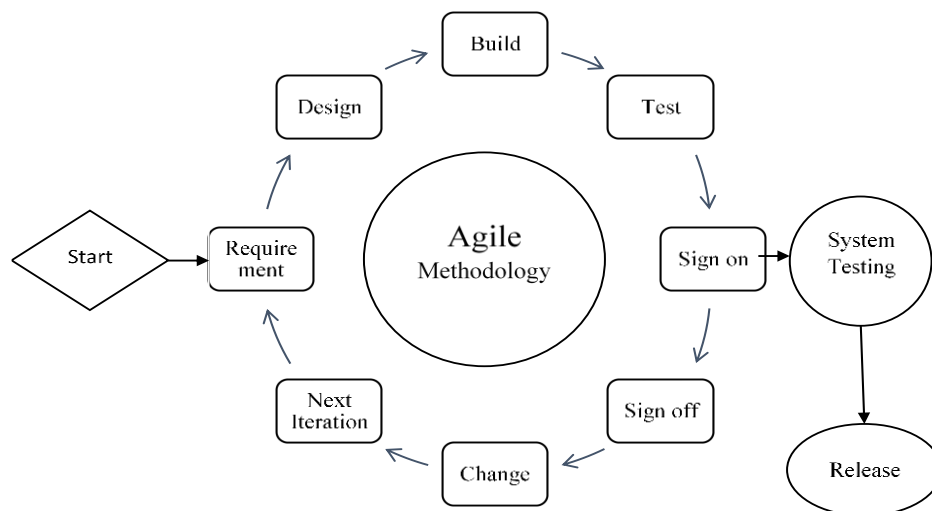
Figure 3.1: Agile Model
