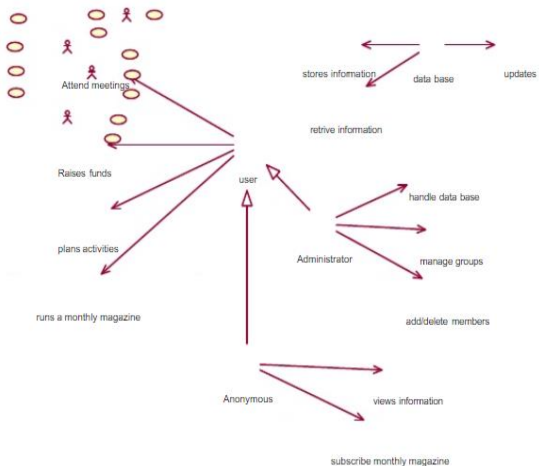
Figure 3.6: Use-case Diagram
