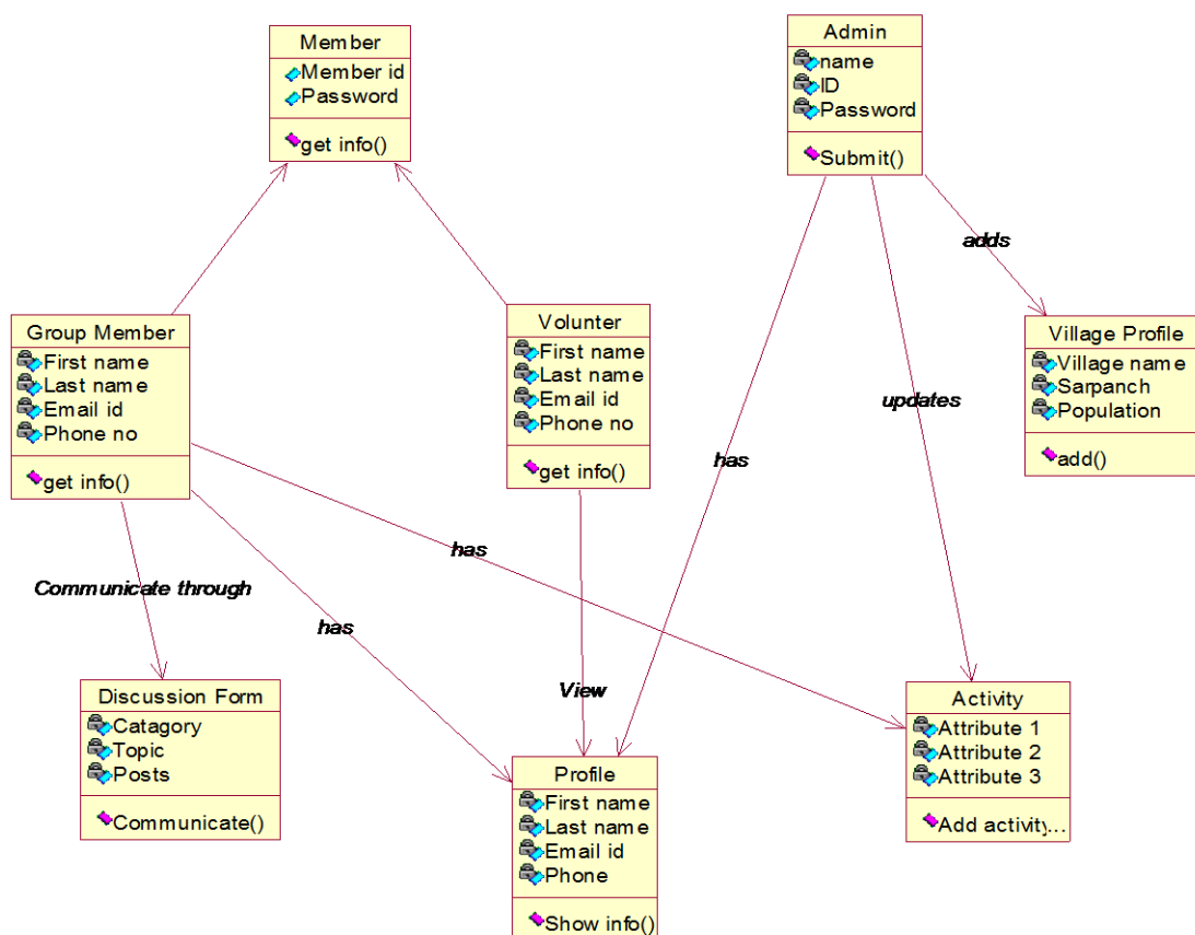
Figure 3.7: Class Diagram
