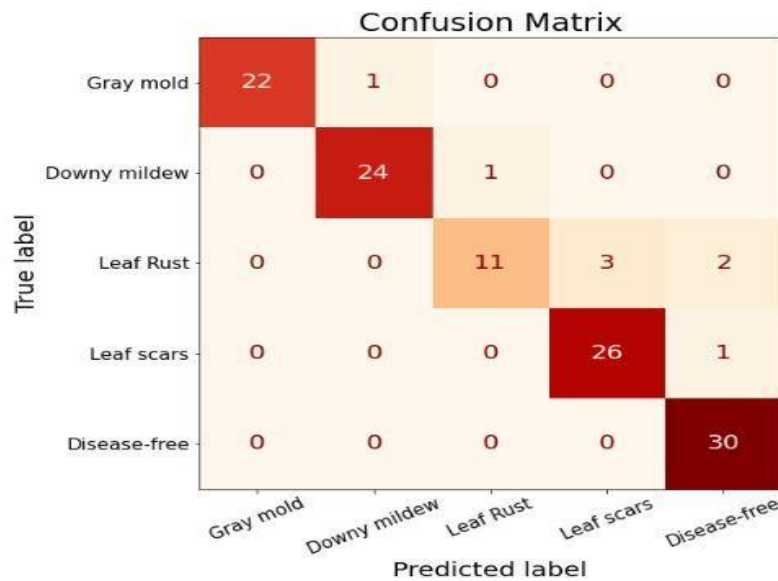
Figure 4.7: Gradient Boosting Confusion Matrices
