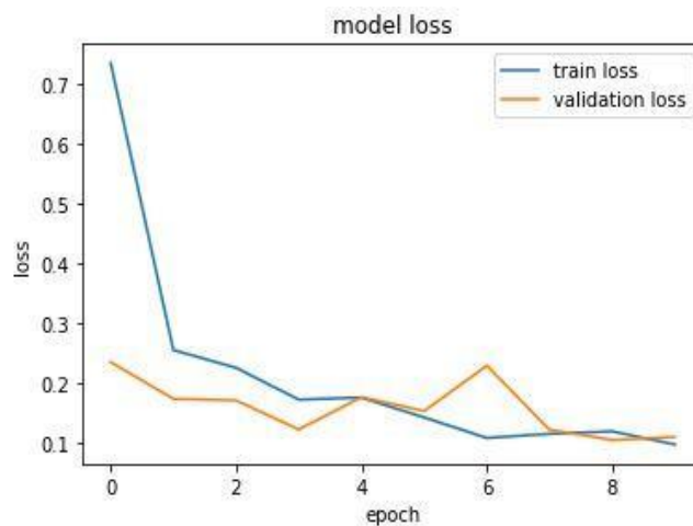
Figure 4.15: ResNet 50 Model Loss Train Loss vs Validation Loss
