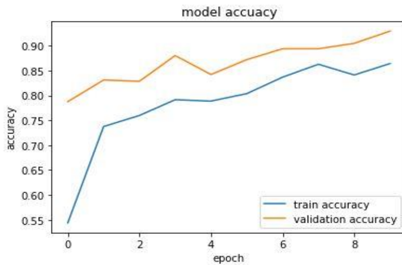
Figure 4.17: VGG 19 Model Accuracy Curve Training Accuracy vs Validation Accuracy
