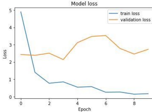
Figure 4.21: MobileNet V2 Model Loss Curve Training Accuracy vs Validation Accuracy
