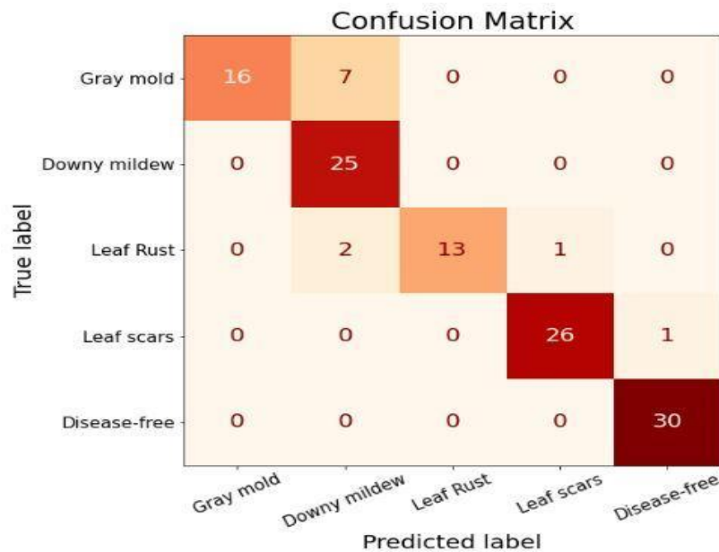
Figure 4.9: K-Nearest Neighbors Confusion Matrices
