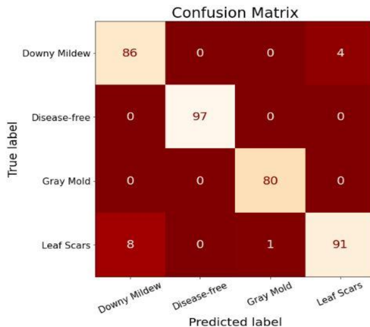
Figure 4.13: ResNet 50 Confusion Matrices
