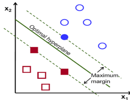
Figure 3.5: Support Vector Machine hyper plane
