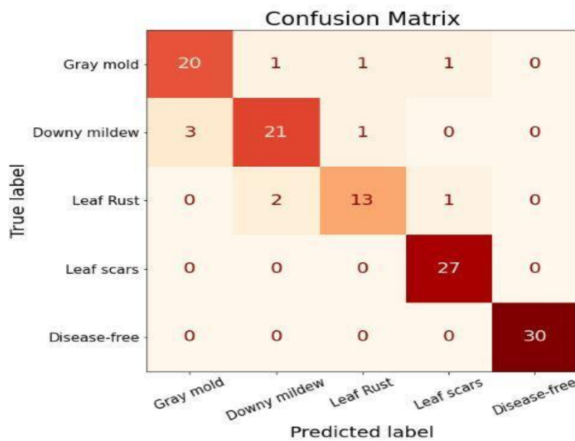
Figure 4.3: Confusion Matrices of Random Forest
