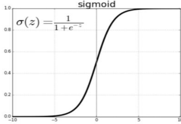
Figure 3.3: Logistic function
