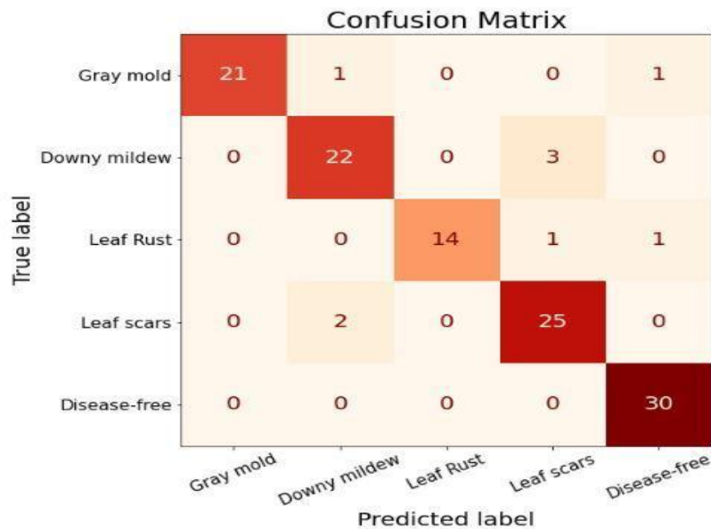
Figure 4.11: XGBoost Classifier Confusion Matrices
