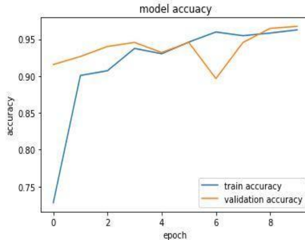
Figure 4.14: ResNet-50 Model Accuracy Train vs Validation
