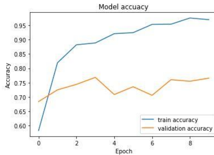
Figure 4.20: MobileNet V2 Model Accuracy Curve Training Accuracy vs Validation Accuracy
